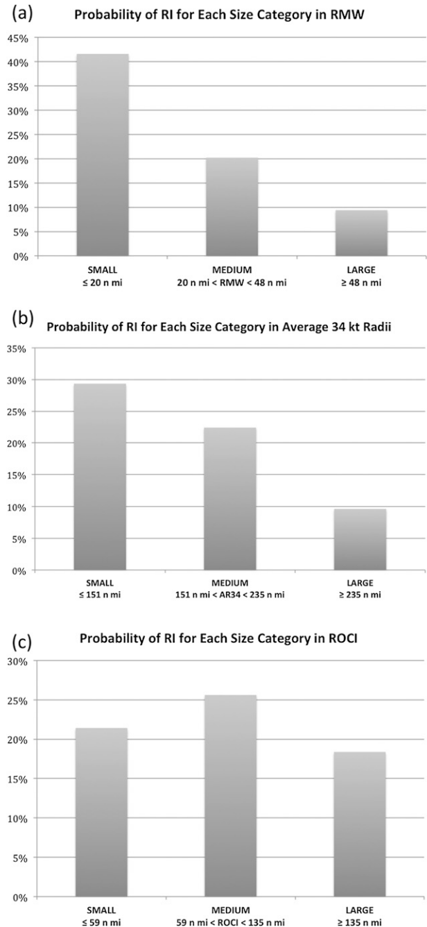
FIG. 4. Probabilities of RI for each size stratification for (a) RMW, (b) AR34, and (c) ROCI.
